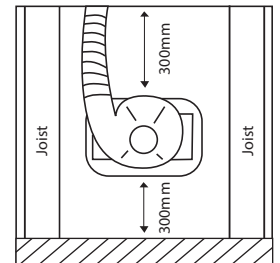
Fig.5 Thermal Insulation
